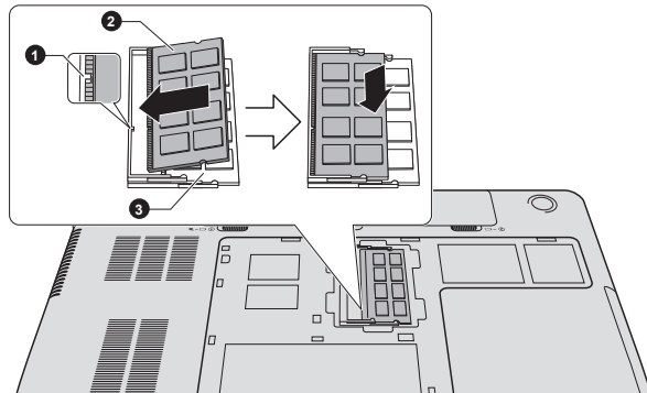
Figure 3-14 Seating the memory module
